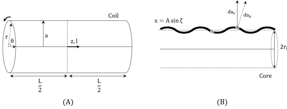
Fig. 2. Illustration of elements of coil and core geometry: (A) the coil has radius a and the axial distance is measured from the midpoint along the axis, (B) the coil has an unperturbed radius r_i , with the area element ascertainable at any random point along the axis, with the fluctuation being characterized by amplitude A and phase \zeta .
