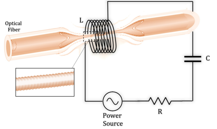
Fig. 1. The scheme for quantum transduction using optoelectromechanical coupling of light in an optical fiber with a microwave signal through the acoustic mode generated in Brillouin scattering in a rare-earth aluminosilicate glass microwire. In this setup, the tapering of an optical fiber carrying the optical signal comprises of the microwire, which is taken as the core of a coil-inductor that is part of microwave resonator RLC circuit. The variation of the cross-sectional area temporally, due to the acoustic mode, leads to variations of magnetic flux and, as a result, the electrical response in the microwave resonator.
